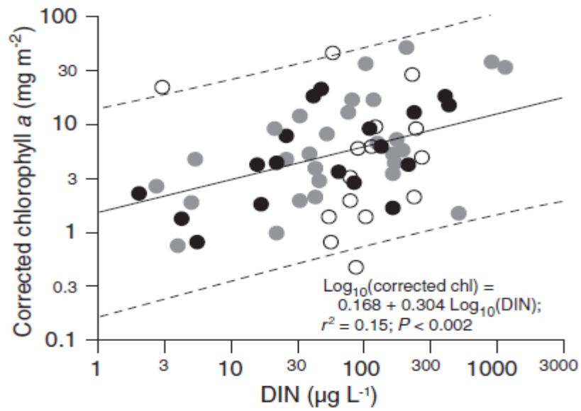
Fig. 5 Frequency distribution of chlorophyll a corrected to a common date and elevation (above) and relationship of corrected chlorophyll a to dissolved inorganic N (below). Corrected chlorophyll is not related to any other nutrient fractions.
