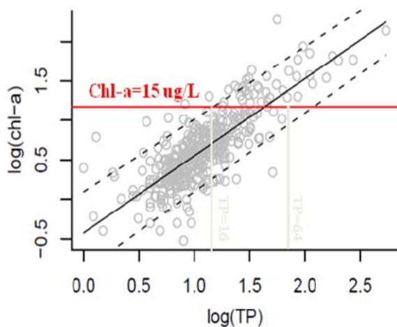
Figure 15. Log(TP) vs. log(chl a ) for EMAP Northeast Lakes Survey. Dashed lines are the 5th and 95th percentile estimated by quantile regression. Solid line is the 50th percentile. Red line indicates where chlorophyll a = 15 µg/L. Units are µg/L.
